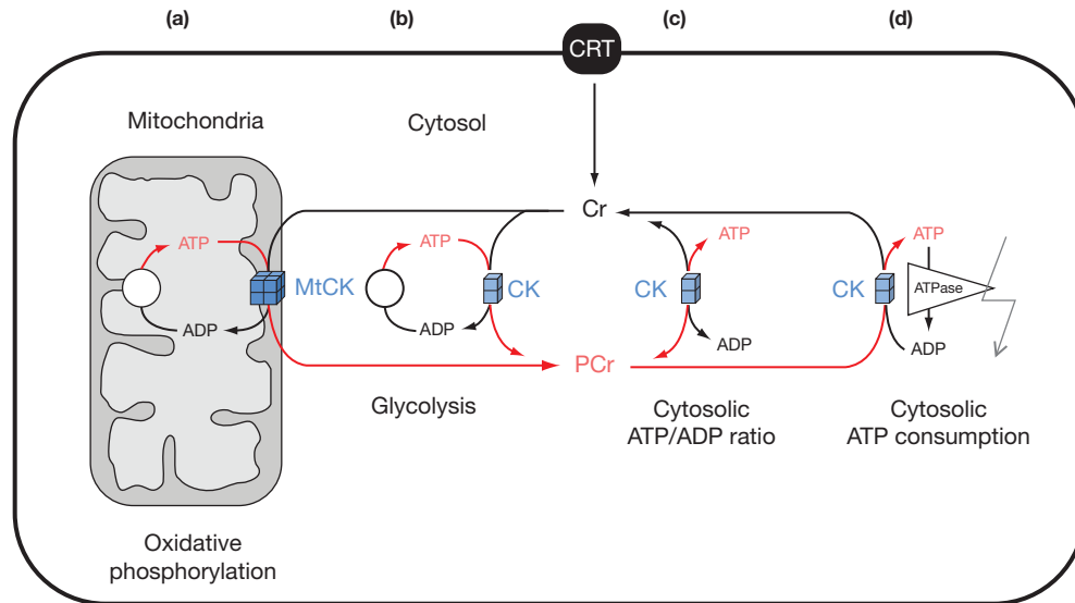
Figure 2 The creatine kinase (CK)/phosphocreatine (PCr) system. Isoenzymes of CK (blue) are found in different compartments such as mitochondria (octameric MtCK, (a)) and cytosol (dimeric CK, (b)–(d)) in soluble form (c) or associated to a different degree to ATP-delivering ((a) and (b)) or -consuming processes (d). A large cytosolic PCr pool up to 30 mM is built up by CK using ATP from oxidative phosphorylation like in heart (a) or glycolysis like in fast-twitch glycolytic muscle (b). PCr is then used to buffer global (c) and local (d) ATP/ADP ratios. In cells that are polarized and/or have very high or localized ATP consumption, these CK isoenzymes, together with easily diffusible PCr, also maintain an energy shuttle between ATP-providing or -consuming processes ((a) and (d)). Metabolite channeling occurs where CK is associated with ATP-providing or -consuming transporters, pumps, or enzymes ((a), (b), and (d)). Creatine (Cr) is synthesized in only few cell types (e.g., liver and kidney) and has to be taken up from the blood stream by a specific Cr transporter (CRT) that is highly expressed by Cr-containing target cells.
